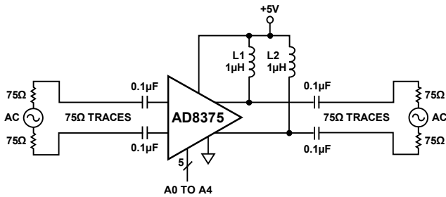
Figure 42. Test Circuit for S-Parameters on Dedicated 75Ω Differential-to-Differential Board
