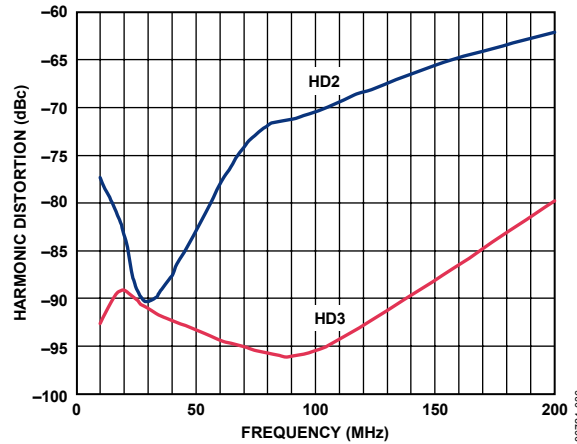
Figure 34. Harmonic Distortion vs. Frequency of Single-Ended-to-Differential Conversion
