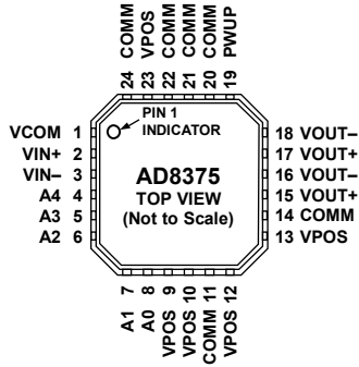
Figure 3. 24-Lead LFCSP
