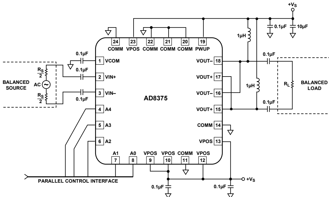
Figure 35. Basic Connections
