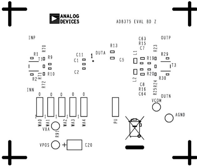
Figure 47. Component Side Silkscreen
