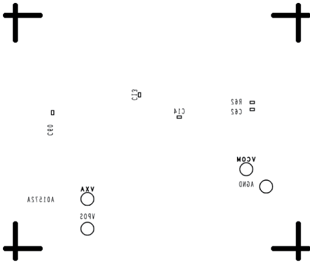
Figure 48. Circuit Side Silkscreen
